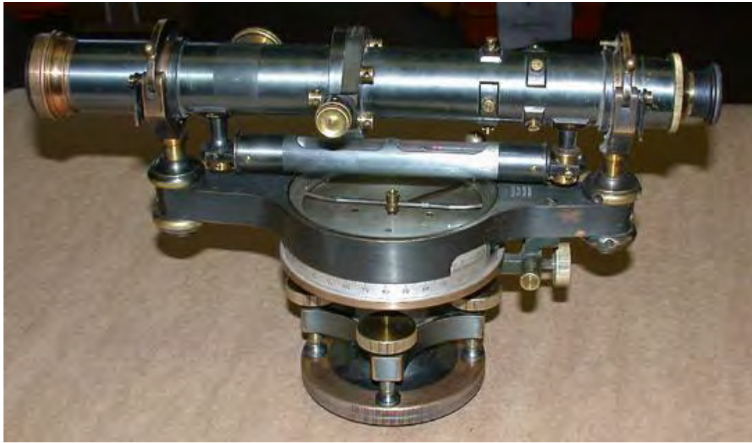
Gambar 1.10. Wye level
